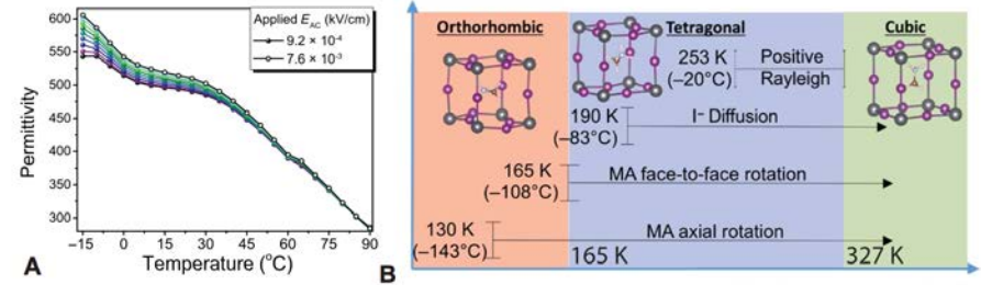
Figure 1. (A) Rayleigh response, determined from the EAC dependence of the permittivity. (B) Schematic of the material structure, temperature dependence of the global phase transitions, possible mechanisms of structural modification, and Rayleigh response in MAPbI 3 .
